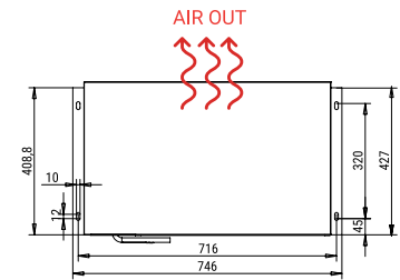
TOP VIEW VISTA IN PIANTA
