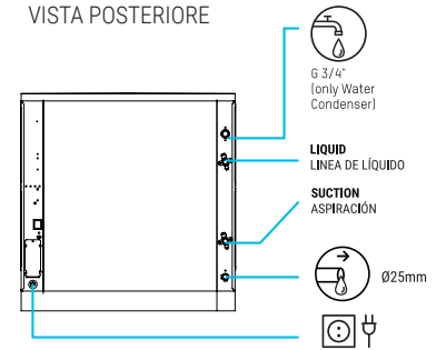
REAR VIEW VISTA POSTERIORE
