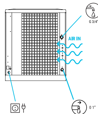
REAR VIEW VISTA TRASERA
