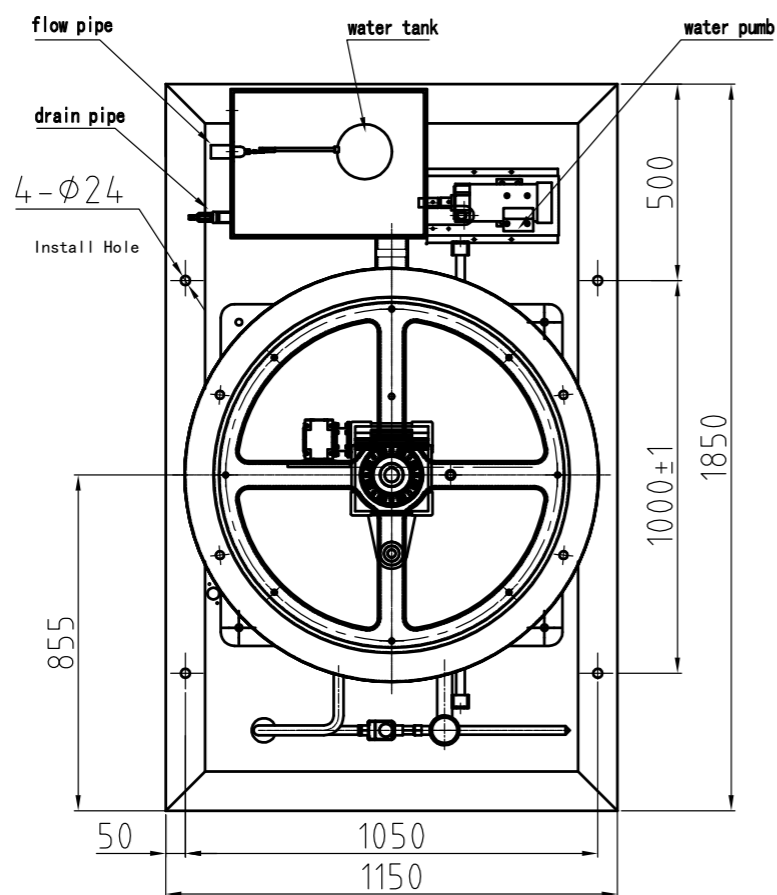
pipe connection drawing (planform)
